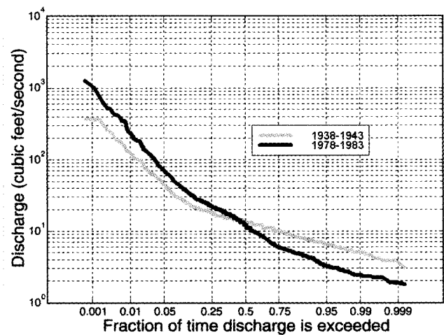
Figure 4. Change in flow distribution in Northwest Branch watershed, Maryland, due to urbanization. The light gray trace shows the flow distribution of mean daily discharges from 1938 to 1943. The black trace shows the flow distribution from 1978 to 1983.
