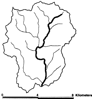
Figure 7. The Northwest Branch watershed is shown with the selected flowpath indicated by the heavy solid line. Streamflow conditions at all points along this flowpath are then illustrated in Figure 8.
