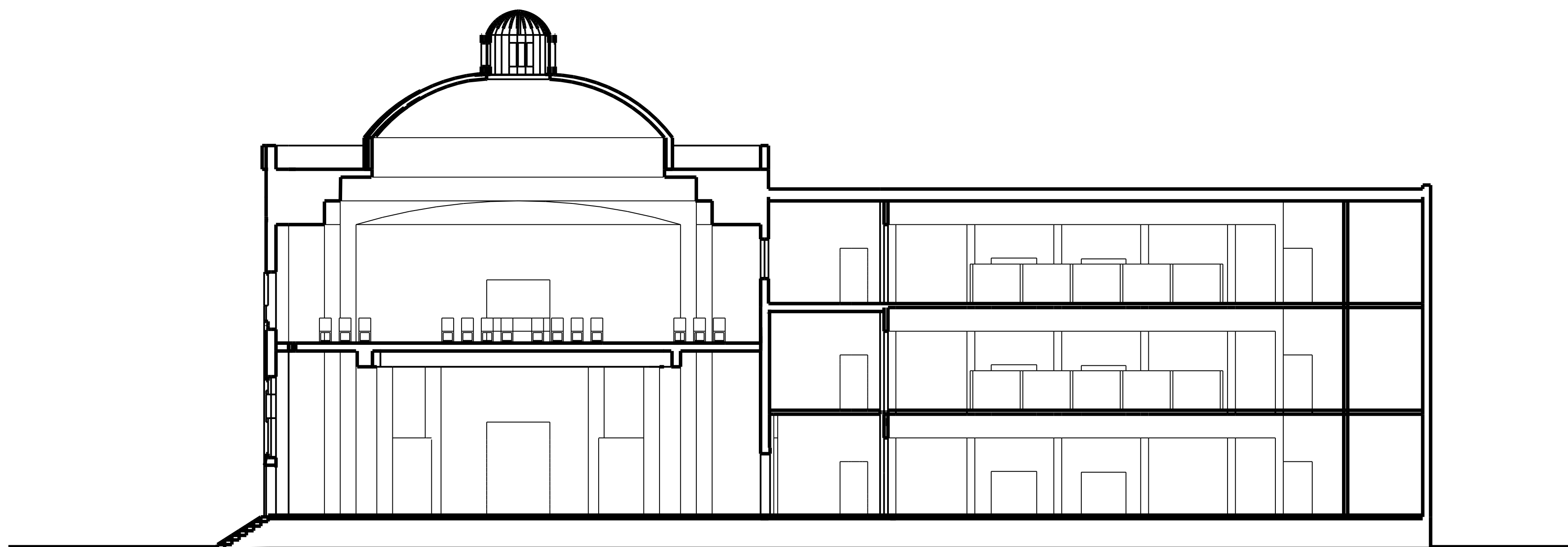
Transverse Section- N/S
